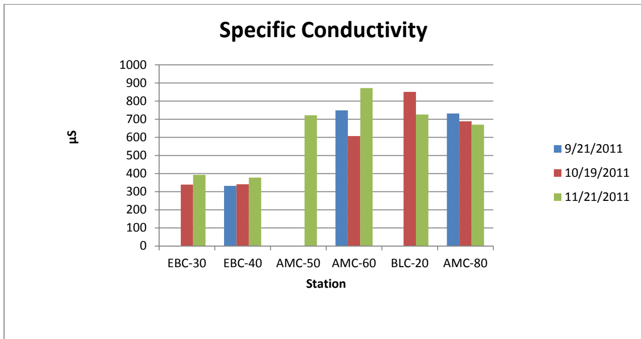
Figure 5: Specific Conductivity Measurements
