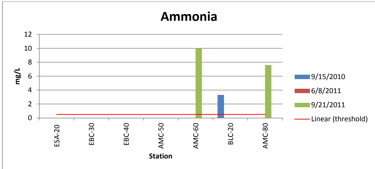
Figure 10: Ammonia Measurements
