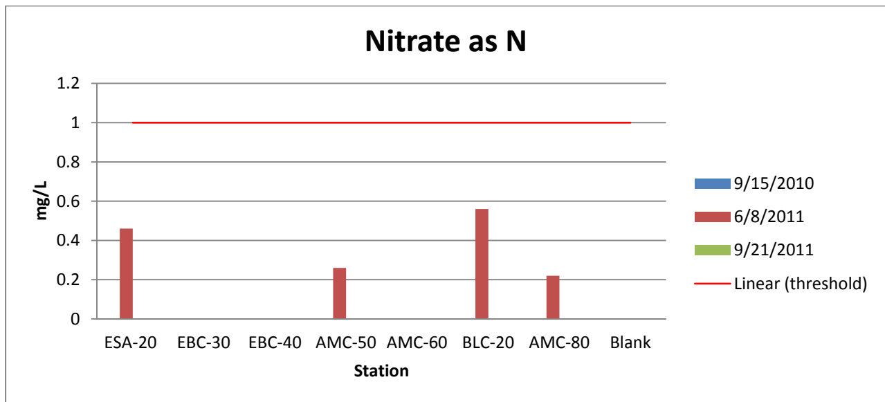
Figure 9: Nitrate Measurements
