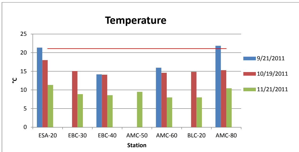
Figure 4: Temperature Measurements
