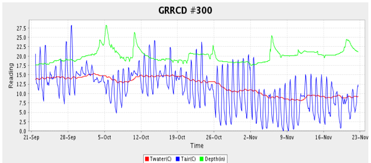
Figure 1: Hydrograph of Salmon Creek from September 21 to November 23, 2011
