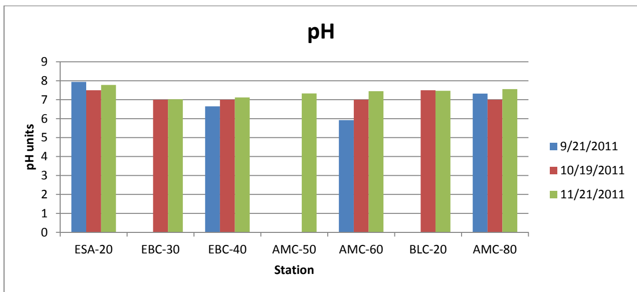
Figure 8: pH Measurement
