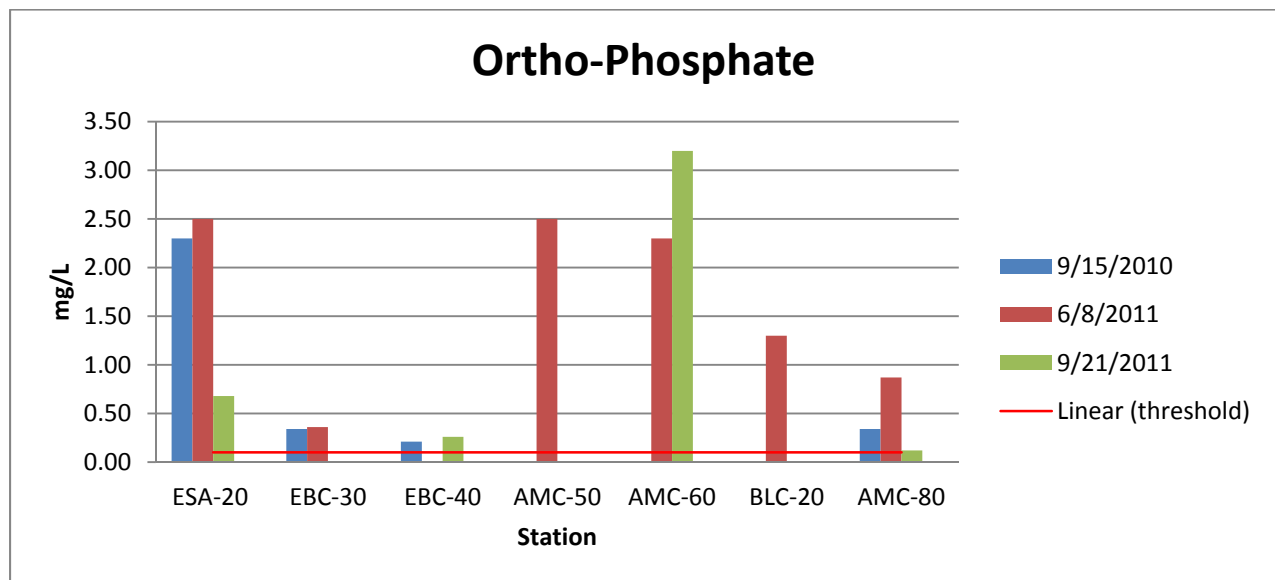
Figure 11: Orthophosphate Measurements
